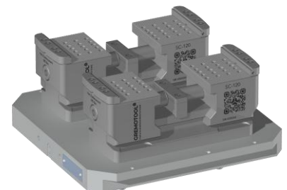
2x SC-120 & System 3R Delphin 398 Pallet
