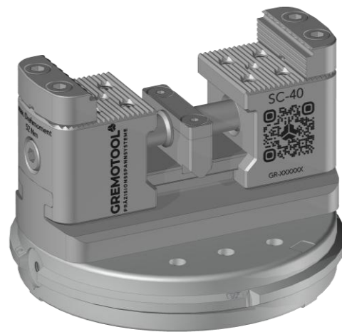
SC-40 & System 3R GPS-120 Pallet
